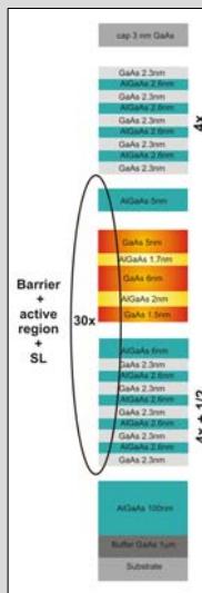
Fig 8. Scheme of Quantum Cascade Laser (QCL) structure grown at Molecular Beam Epitaxy Laboratory (left). The Photoluminescence Excitation (PLE) map of QCL active region structure detected at 1,583eV [1e-11h] (right).
