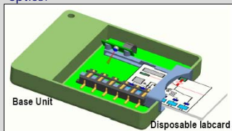
Concept of OPTOLABCARD hand held base unit and a labcard (left) and scheme of the card (right) integrating microfluidical, optoelectrical and microbiological devices
