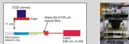
Measurement set-up of the detection unit with CCD camera/filter module: scheme (left) and real picture (right) of the stand
