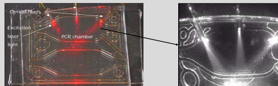
Top views of PCR chip made of glass and SU8, developed by MIC (Technical University of Denmark), on the testing stand (left) and real picture of the sample, containing 250 ng/ml of salmon sperm DNA labelled by TO-PRO 3 fluorochrome, irradiated simultaneously by three optical fibres, the picture captured by CCD camera equipped with 650 nm long-pass filter (adjusted to emission wavelength of TO-PRO 3 fluorochrome)
