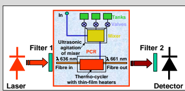
Concept of OPTOLABCARD hand held base unit and a labcard (left) and scheme of the card (right) integrating microfluidical, optoelectrical and microbiological devices
